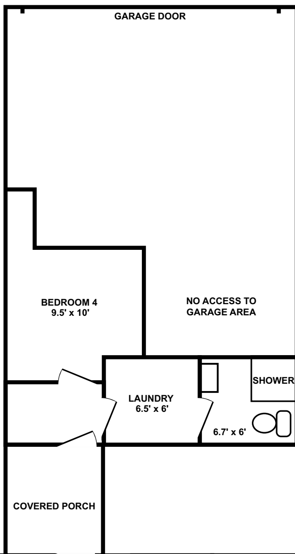
PIER 121 FLOOR PLAN
